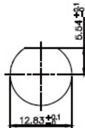
RECOMMENDED MOUNTING HOLE MAXIMUM PANEL THICKNESS: 5.5MM
