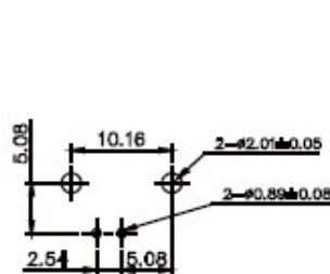
RECOMMENDED PC BOARD LAYOUT WITHOUT MOUNTING POSTS
